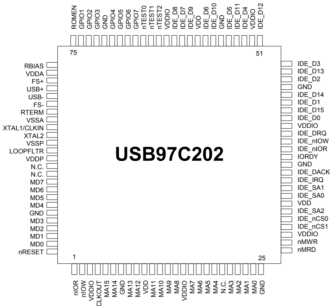
Figure 3.1 - 100 PIN STQFP
